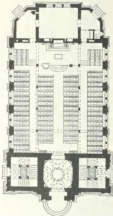
Ground-Plan of the Synagogue at Reichenberg, Bohemia.
